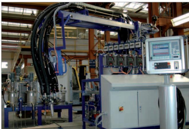
The multi-component PU-processing machine has been in operation at Kobra since April 2007.
