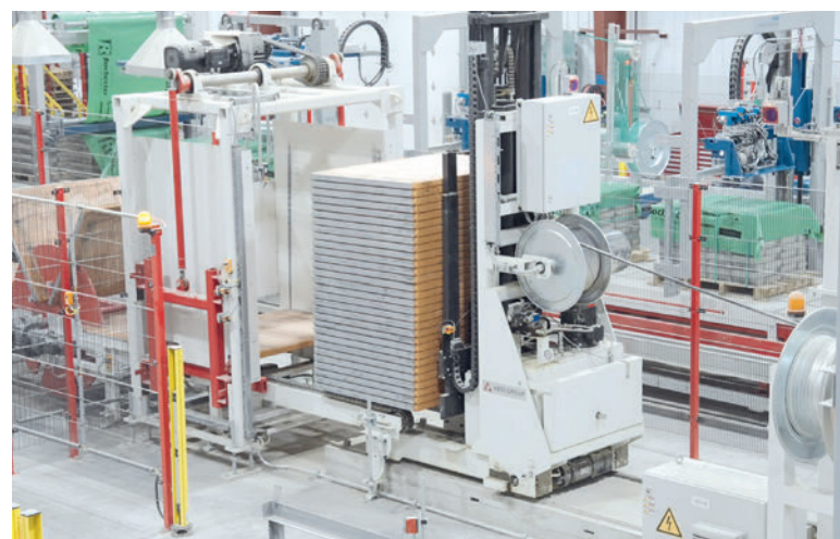
The board buffer cart automatically collects, stores, and transfer production board to machine on demand.
