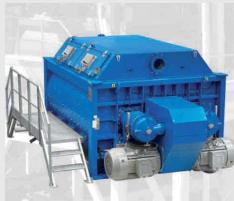
MAO Twin shaft mixer up to 9 m 3 compacted output
