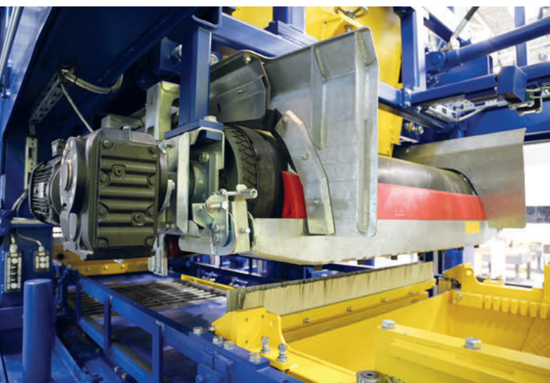
Dosing belts enable variable and optimal filling of the main and face mix filling box
