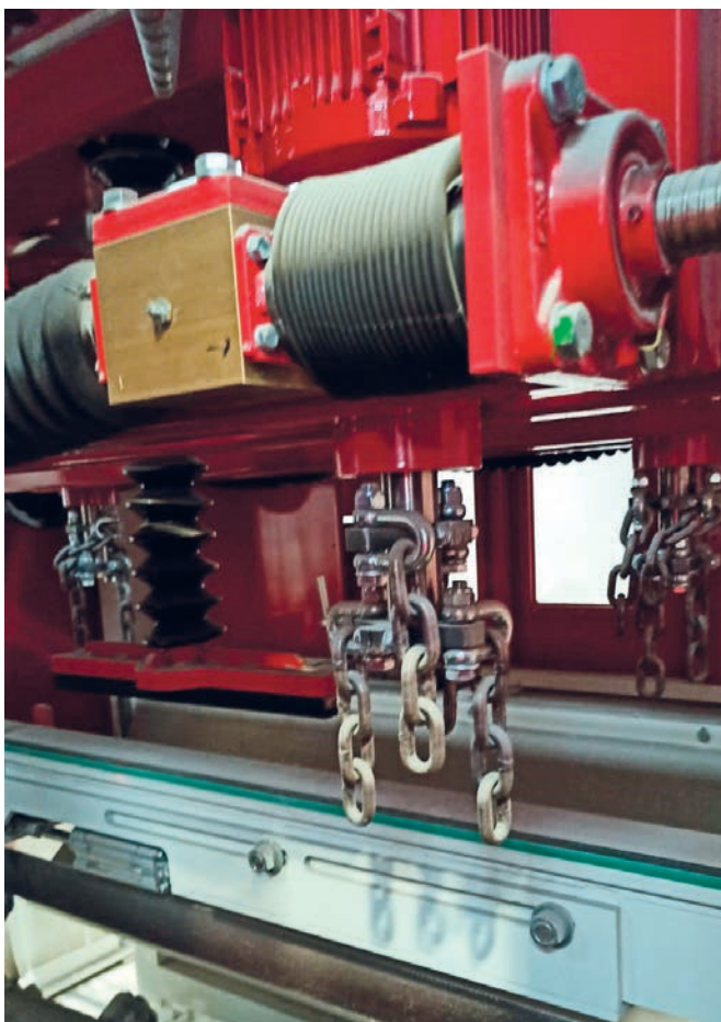
Chain impact supports for processing vertical edges
