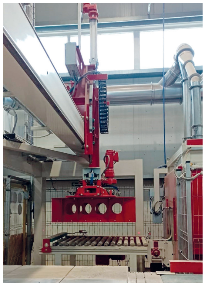
Transfer unit with pneumatic 2-sided clamp
