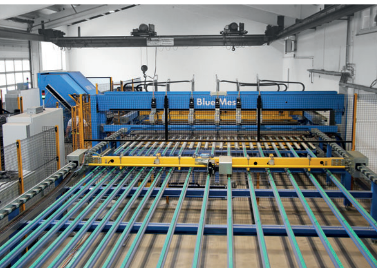
The new M-System BlueMesh® mesh welding system makes it possible to produce made-to-measure reinforcing meshes flexibly
