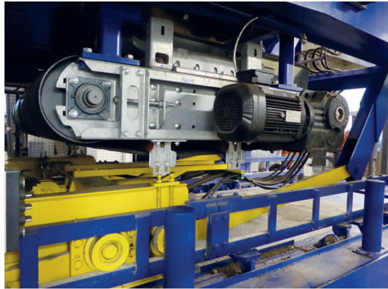
Optional add-on-package: dosing belt
