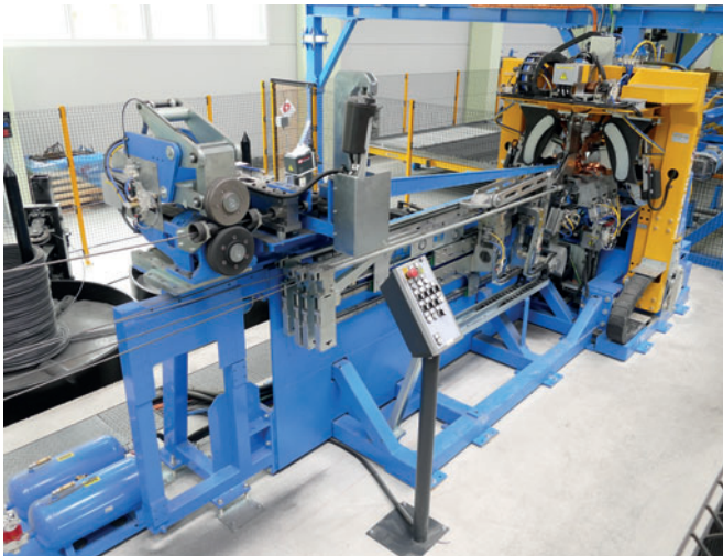
With the highly flexible VGA Versa lattice girder welding machine, the lattice girders are produced "just in time", which enables Eder to achieve high savings potential in logistics, storage costs and waste.
