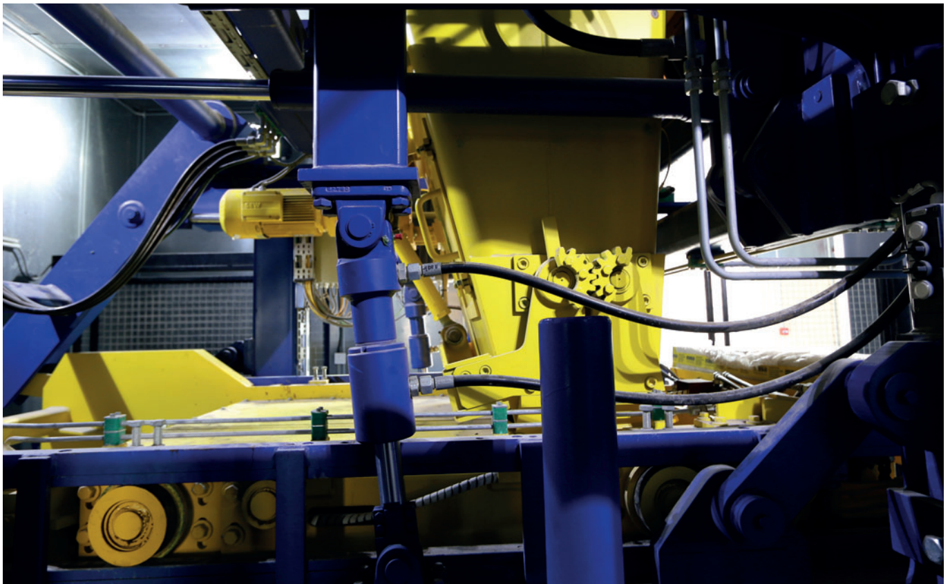
View into the Masa XL - The face mix concrete is dosed directly into the filling box via a silo flap.
