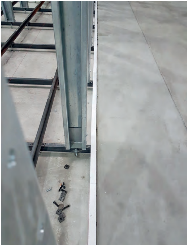
Insulation board is the solution for insulating the perimeter of the curing chamber after installing the rack and rails, but prior to placement of the screeded floor. All steel support beams for the production building must be insulated and isolated from the concrete inside the curing chamber. These steel columns are highly efficient thermal bridges and can cause numerous issues in the way of standing water.
