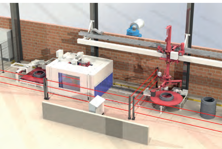
The Prinzing-Pfeiffer pallet line manages the handling of base pallets within the concrete pipe production.
