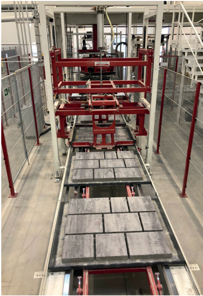
Dry-side transport with 4-sided pusher
