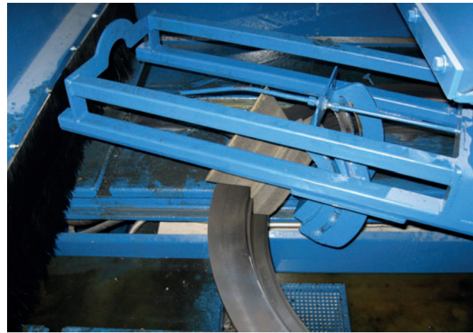
Pallet oiling using a sponge and therefore no spray
