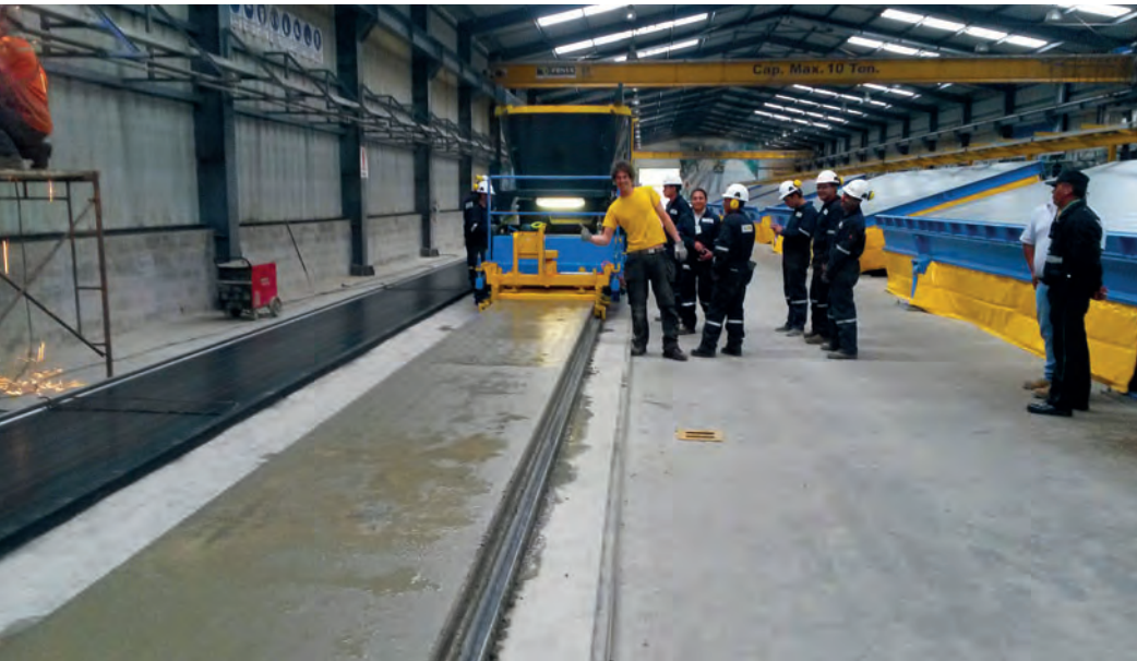
The hollow core slabs are produced on two beds, each 114 m long, with the aid of a slipformer from Echo Precast Engineering.
