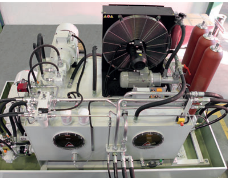
Hydraulikaggregat
