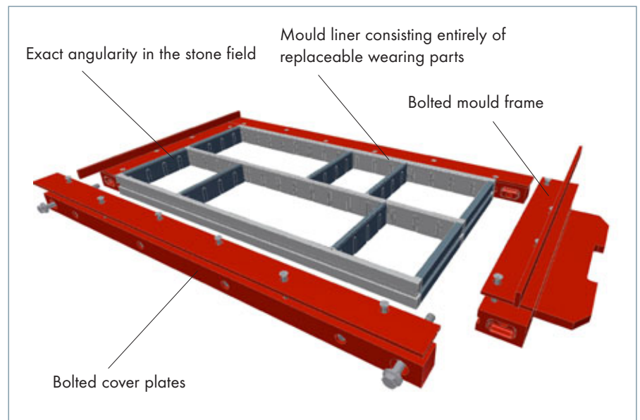
Figure 1: Modular construction method of a Kobra concrete block mould
