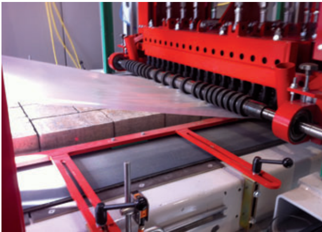
Untreated products at the intake to the aging plant; the synchronously running film protects the product surfaces against damage during the aging process.
