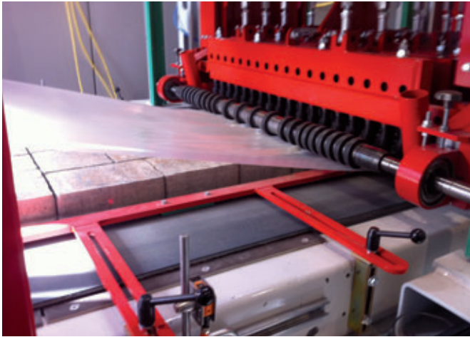
Untreated products at the intake to the aging plant; the synchronously running film protects the product surfaces against damage during the aging process.
