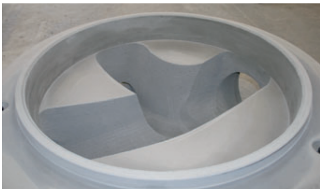
Monolithic concrete manhole base section from the Primuss production line
