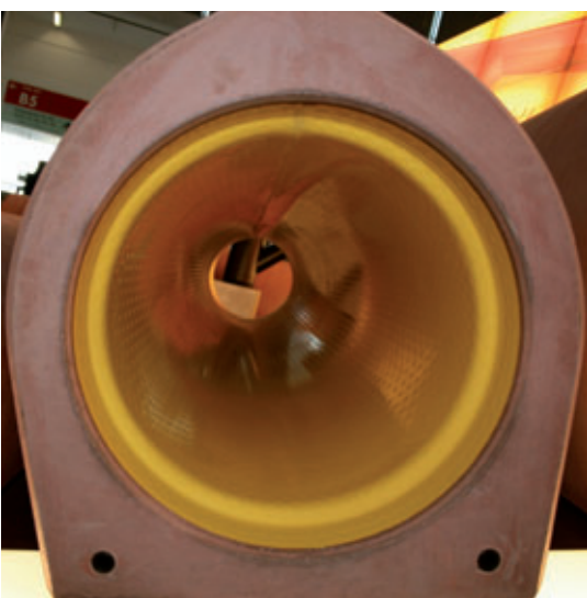
A look at the new concrete-plastic composite pipe Perfect Pipe+
