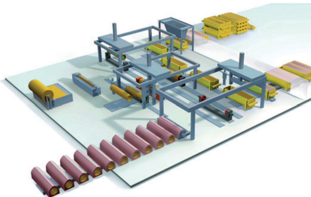
The core of the Perfect Pipe+ production at a glance – economical use of resources and cost-effective processes are crucial
