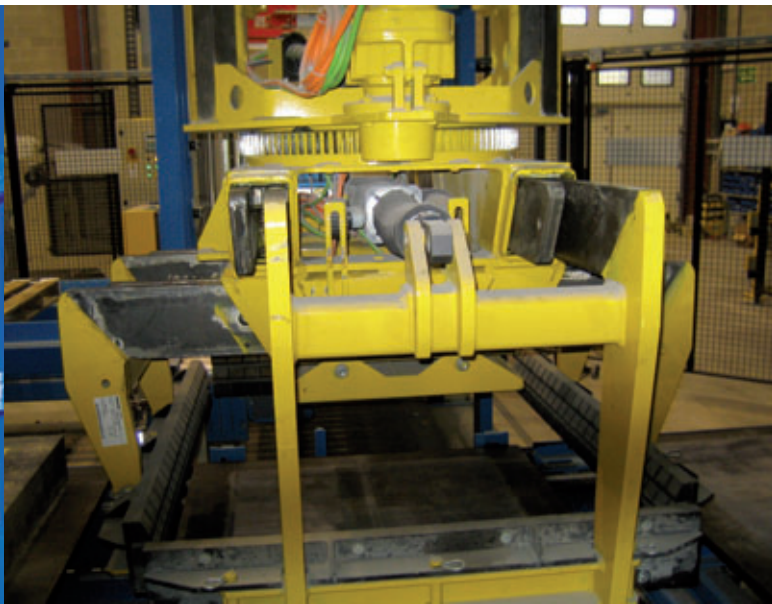
Cubotor with Servo Clamp
