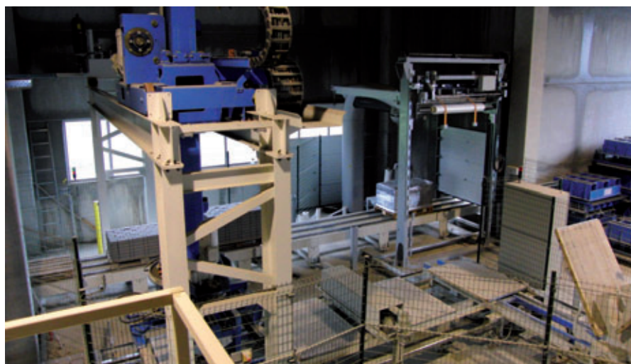
Fig. 5: The packet assembler places the product layers on a transport pallet. A conveyor transports the finished stone packet to a foil wrapping machine and subsequently out of the hall.
